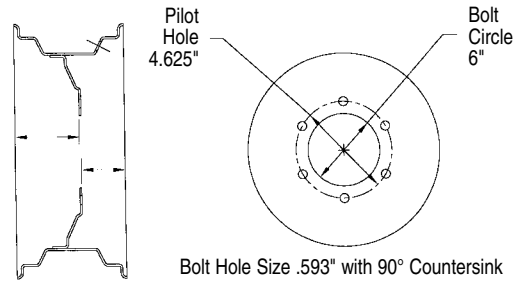
Bolt Hole Size .593" with 90° Countersink
